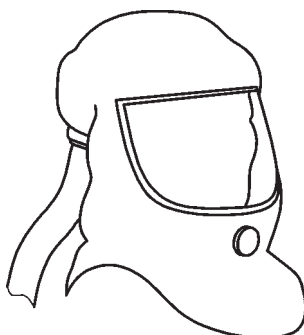
Figure A.9 — Examples of loose-fitting respiratory interfaces covering the head — Class dL
