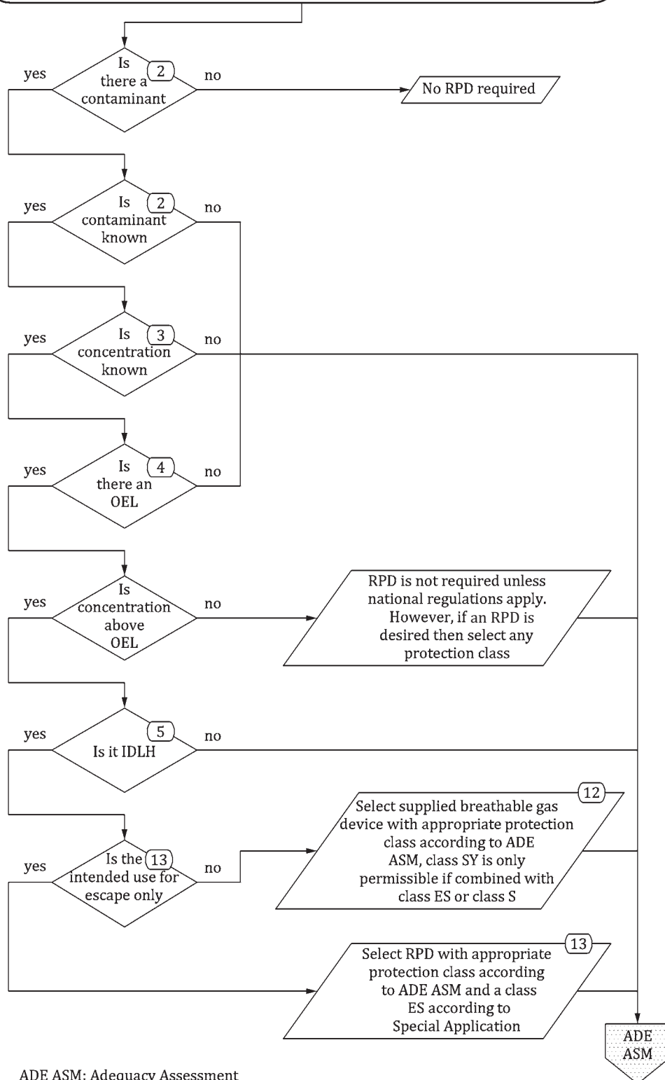
Chart B - Hazard assessment for selection of RPD for oxygen-sufficient atmosphere
